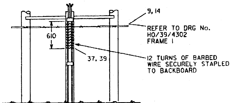
ANTI-CLIMBING
